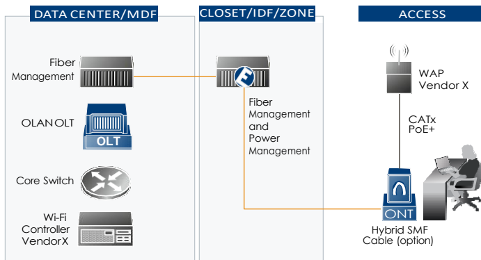
Figure 6: Wi-Fi over Optical LAN architecture
